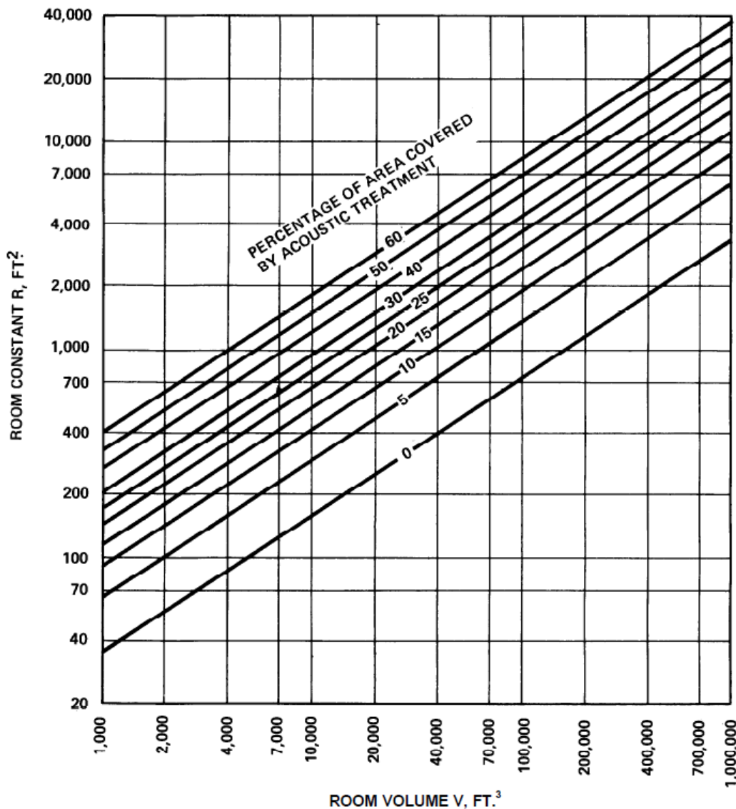
Figure C-2 Room Constant Estimate
