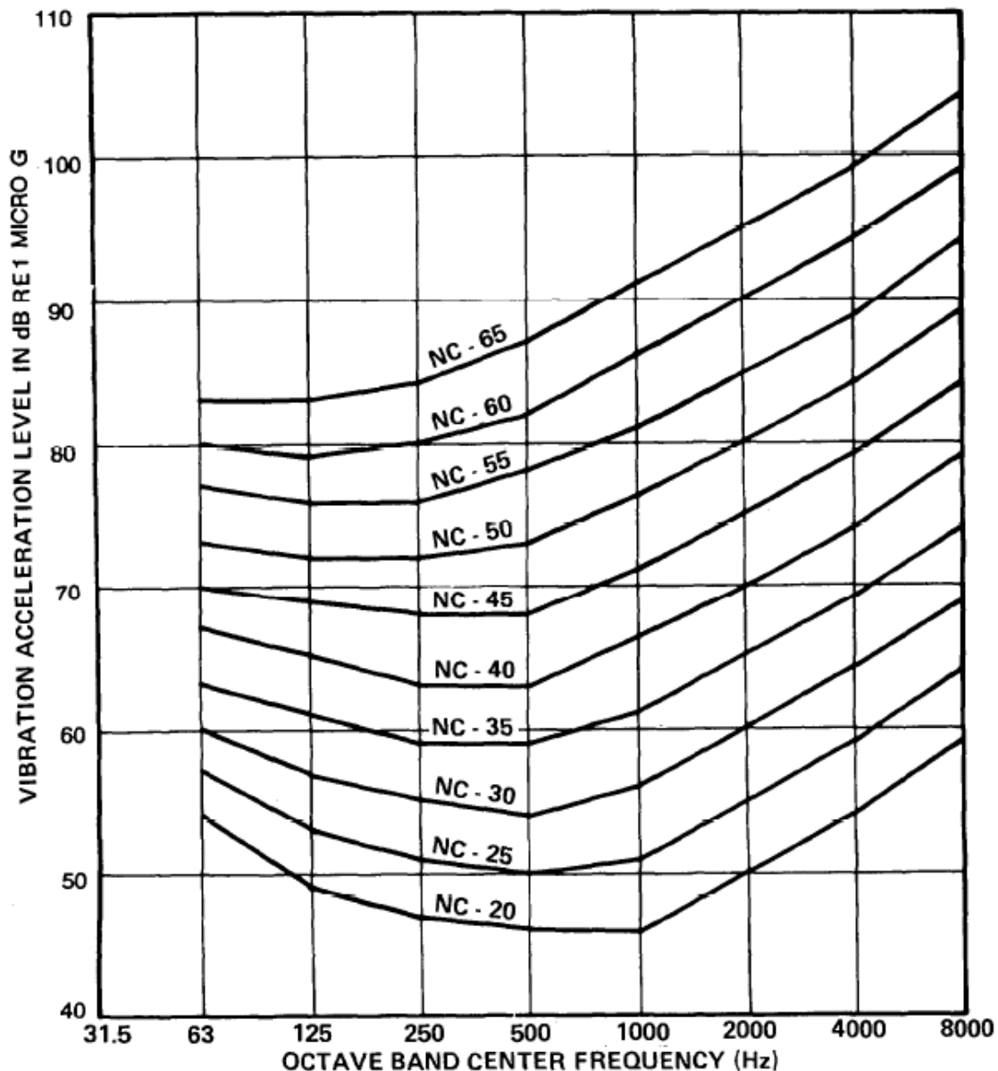
Figure 3-4 Vibration Acceleration Levels of a Large Vibrating Surface that Will Produce Radiated Sound Levels into a Room Approximating the Sound Levels of the NC Curves
