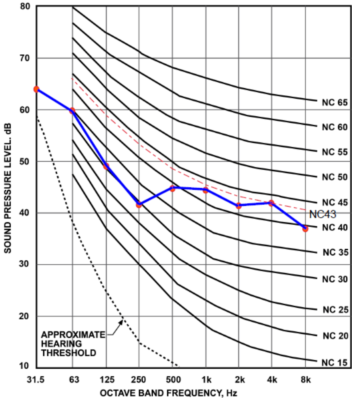
Figure 2-2 Noise Criterion (NC) Curves Tangent Plot.
