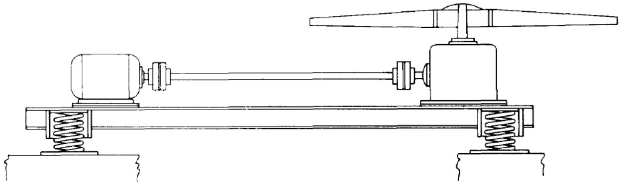
Figure C-23 Schematic of Vibration Isolation Mounting for Fan and Drive-Assembly of Propeller-Type Cooling Tower
