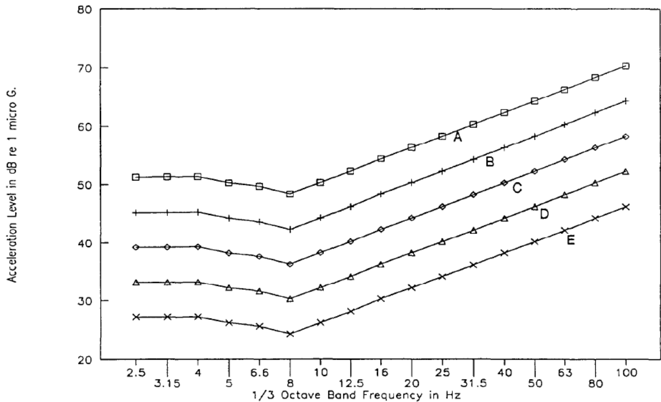
Figure 3-3 Vibration Criteria for Sensitive Equipment in Buildings.
