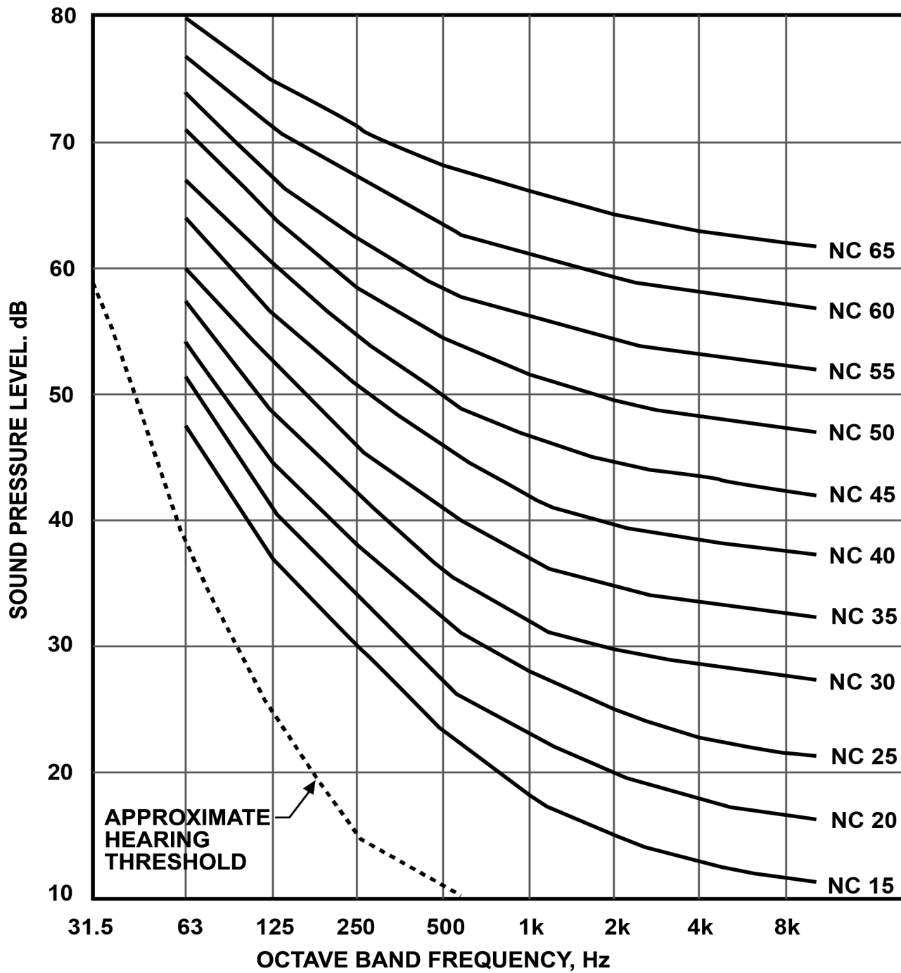
Figure 2-1 Noise Criterion (NC) Curves.
