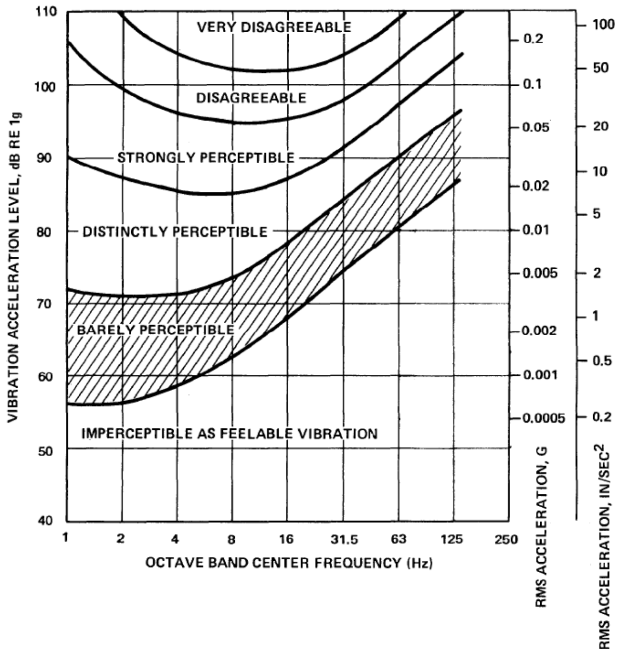
Figure 3-1 Approximate Sensitivity - Response of People to Feelable Vibration
