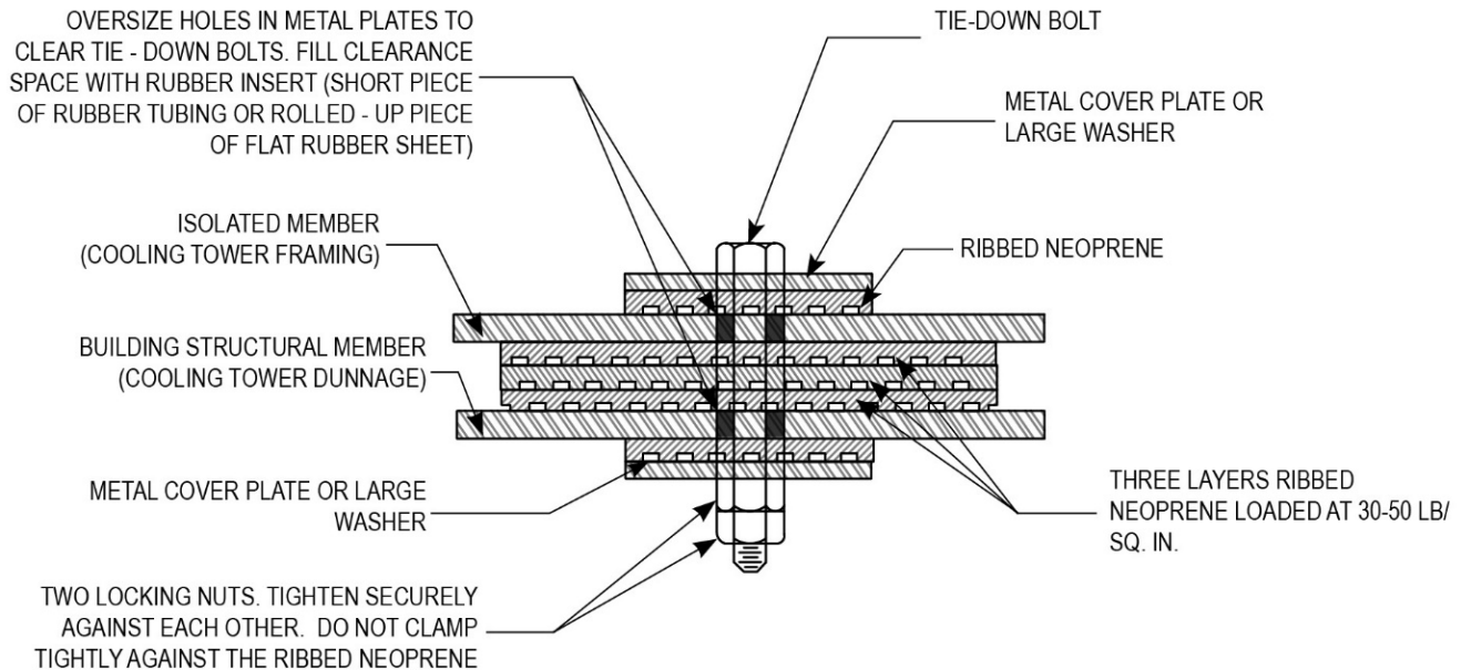
Figure C-24 Schematic of a Resilient Clamping Arrangement With Ribbed Neoprene Pads
