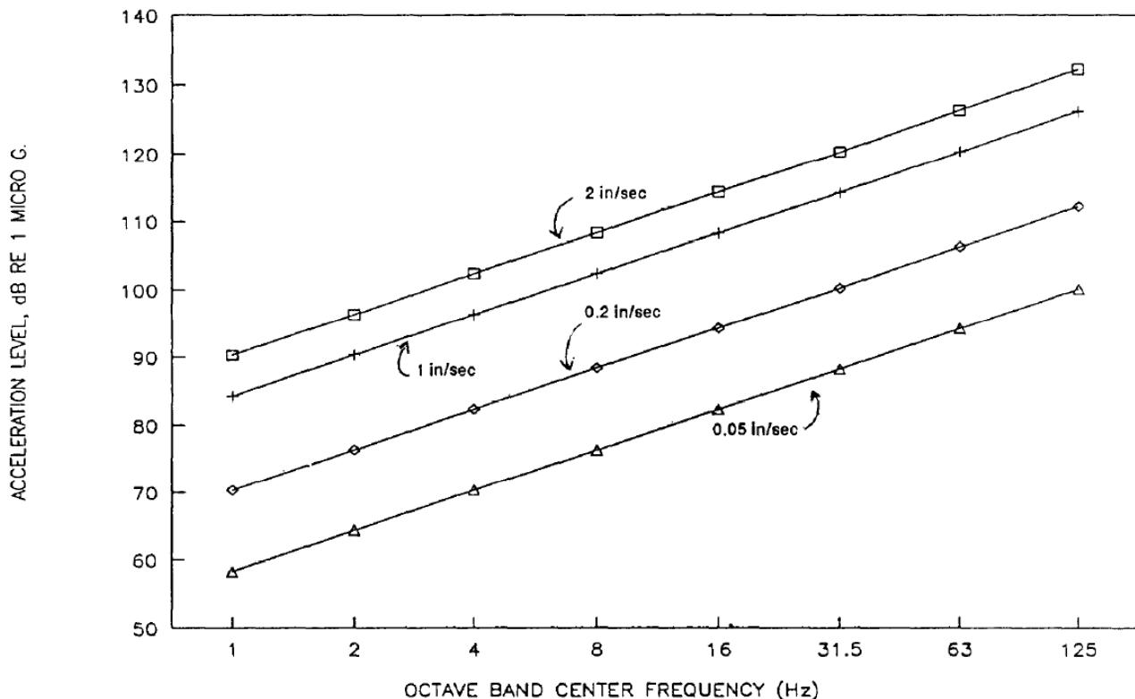
Figure 3-2 Vibration Criteria for Damage Risk to Buildings.
