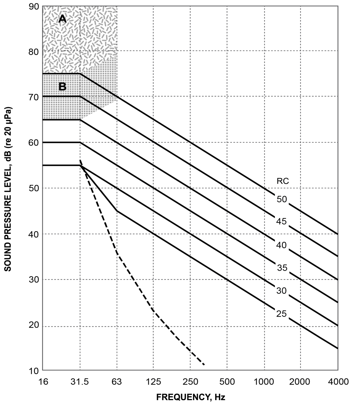
Figure 2-3 Fig 3-3 Room Criterion (RC) Curves, Mark II
