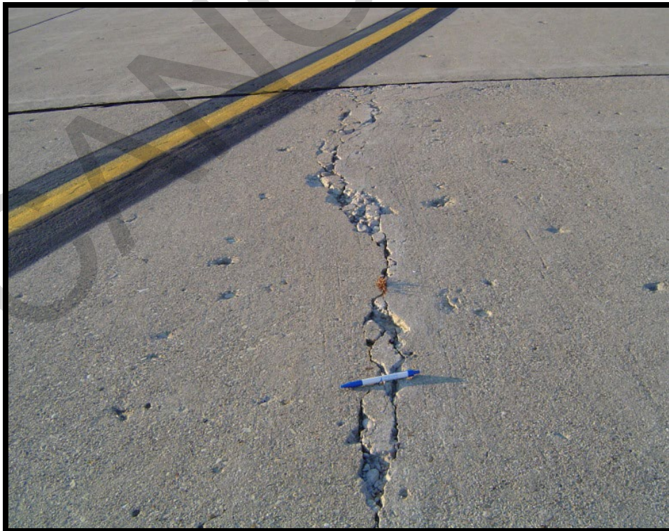
Figure B-10 High-Severity Linear Cracks
